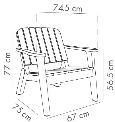
Single Seat
